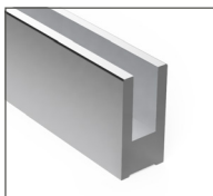
LOW PROFILE BASE CHANNEL (1) 2-3/4" X 1-3/8" CHANNEL MILL FINISH - CLADDING AVAILABLE IN SATIN SILVER OR BRUSHED STAINLESS CAN BE PAINTED OR POWDER COATED Part #: A42-0064AEY10C
