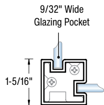
ITEM NO. PP6421000/PP6431000 Partition Corner Post
