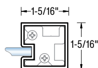
ITEM NO. PP6423000/PP6433000 Partition End Post
