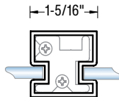
ITEM NO. PP6422000/PP6432000 Partition Center Post
